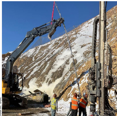
Inserting test pile.
