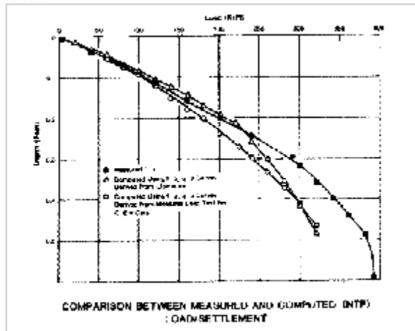
Figure 14. Load/settlement for Natchez Trace Parkway bridge.
