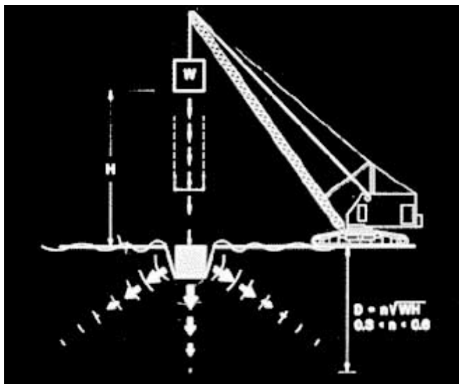
FIGURE 35. Schematic of dynamic compaction methodology.
