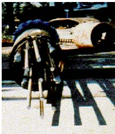
FIGURE 19. Instrumented drilled shaft showing man-made defect and NDE access tubes.
