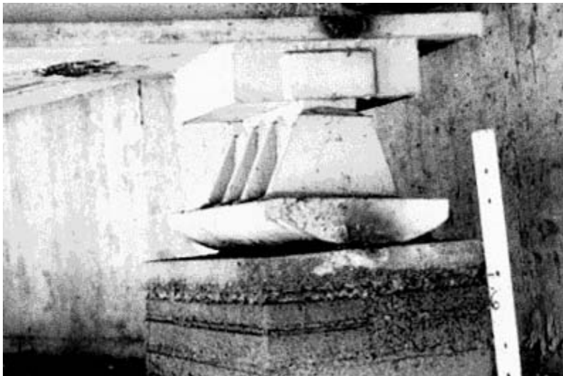
FIGURE 1. Significant shimming beneath bearing device.
