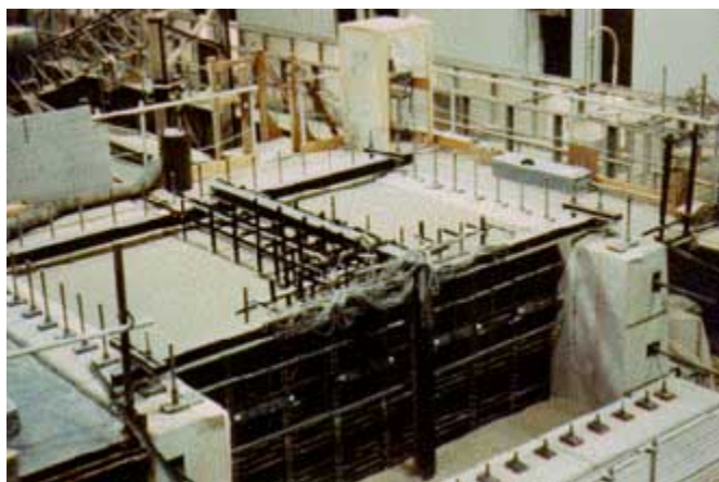
FIGURE 31. Large model ground anchor test wall.
