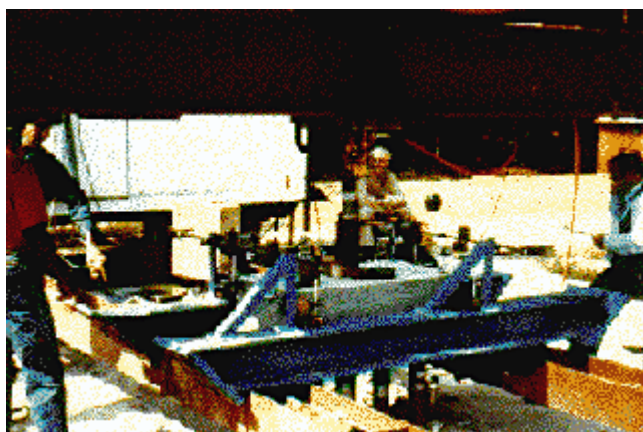
FIGURE 16. Load test on large-scale model pile group in test pit.
