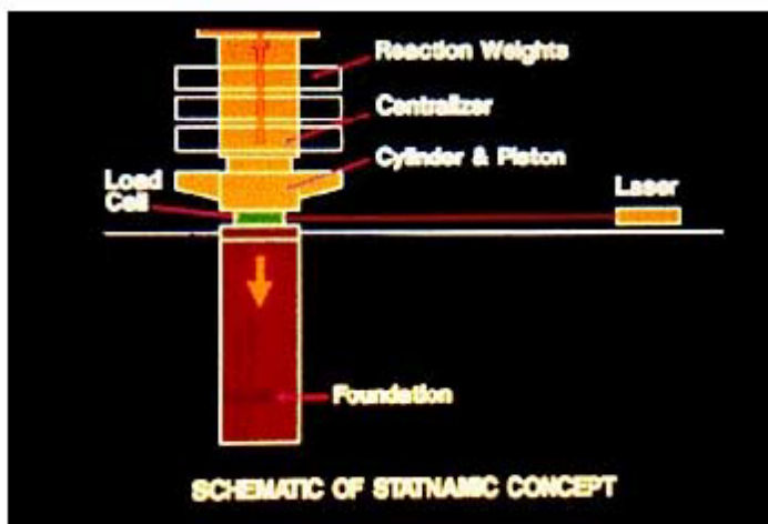
Figure 23. Schematic of statnamic load test method.
