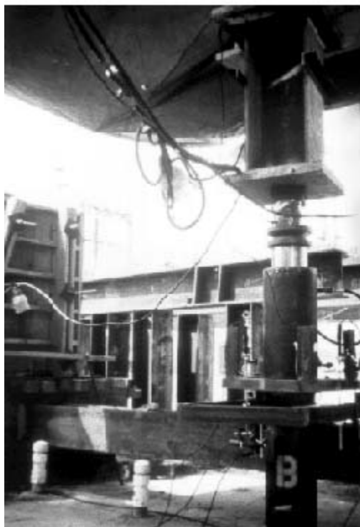
Figure 8. Close-up view of single pile load test in sand.
