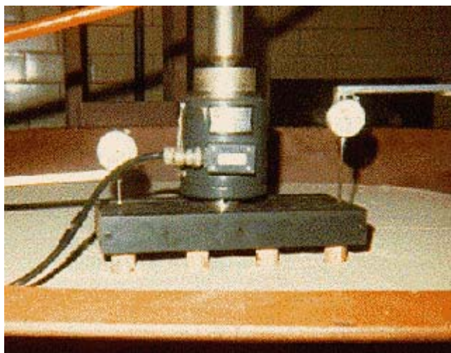
FIGURE 15. Load test on small-scale model pile group in test tank.
