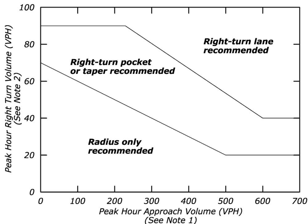
Exhibit 9.3-Q RIGHT-TURN LANE GUIDELINES
