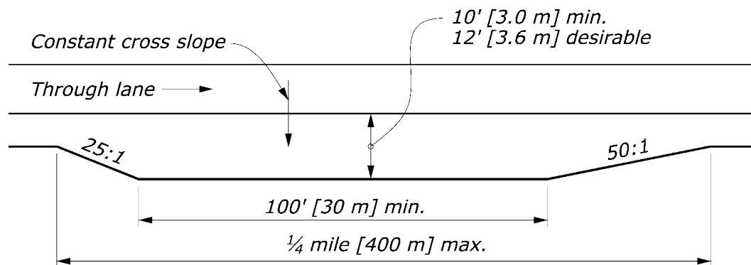
Exhibit 9.3-K SLOW-MOVING VEHICLE TURNOUT
