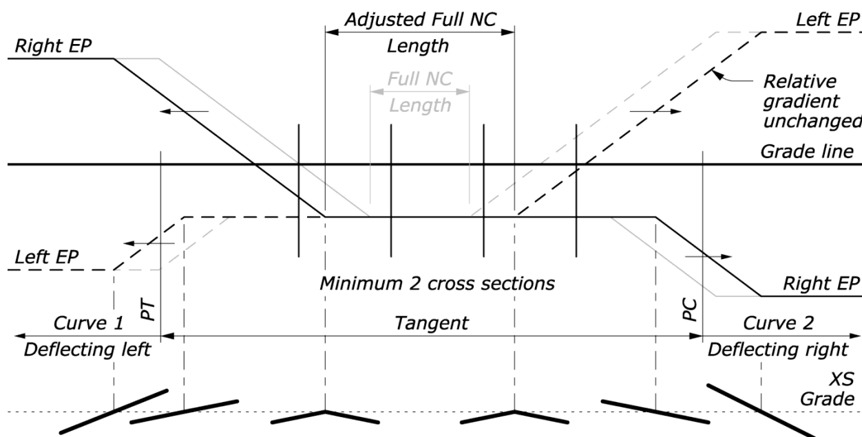
Exhibit 9.3-D TREATMENT OF REVERSE CURVES: CRITICAL CASE
