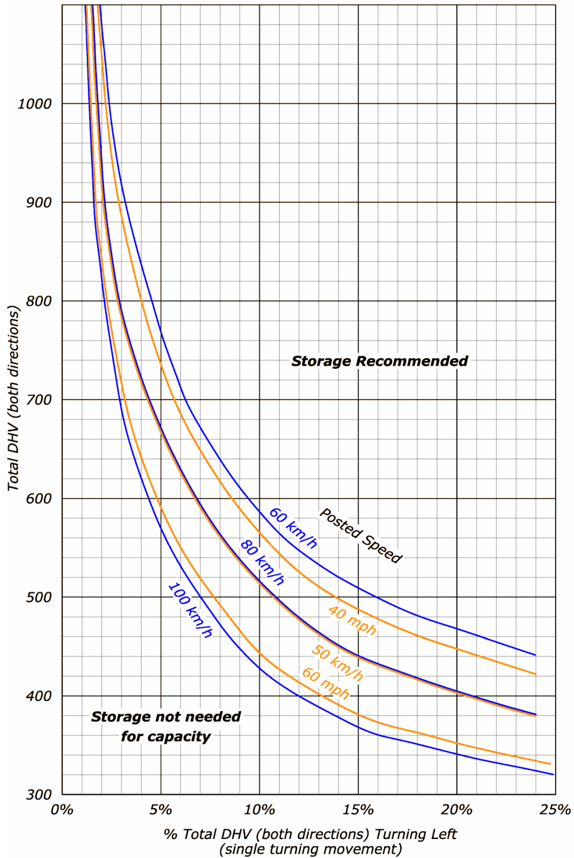
Exhibit 9.3-O LEFT-TURN STORAGE GUIDELINES FOR UNSIGNALALIZED TWO-LANE HIGHWAY INTERSECTIONS
