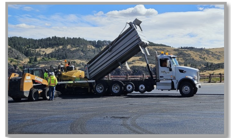
Paving OK-A-BEH Marina Parking Lot
