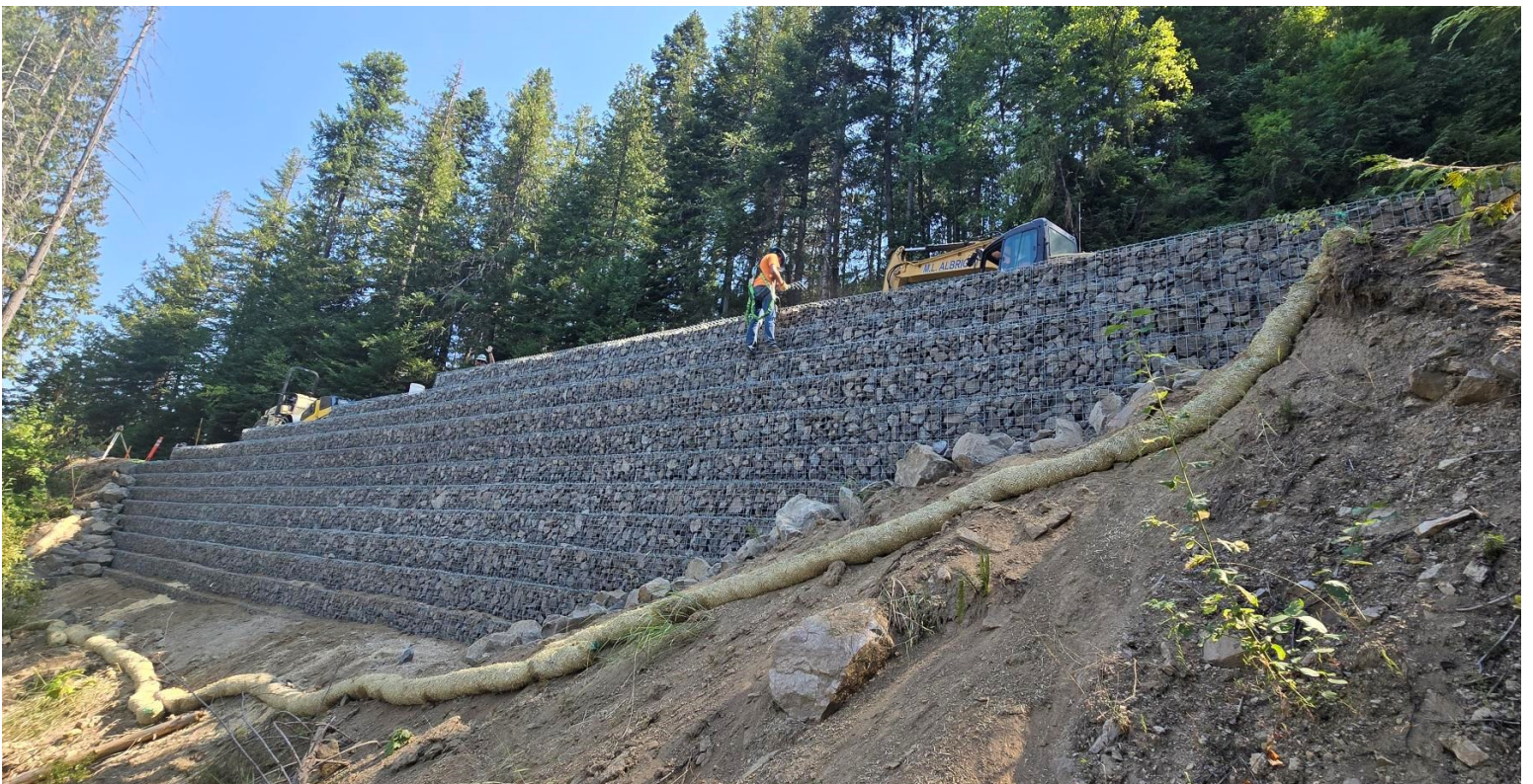
Gabion faced wall construction, M.P. 2.36 FSR 470
