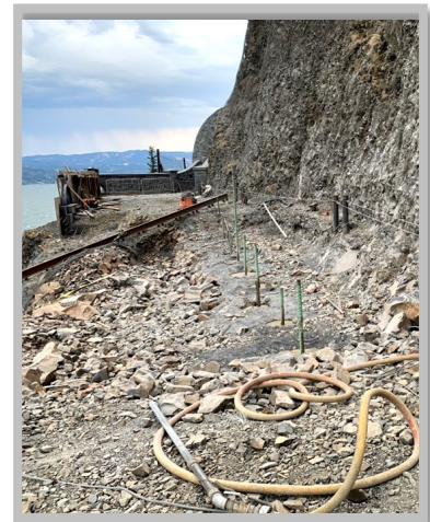
Installation of Ground Anchors in West Bench
