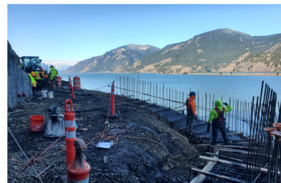
Pouring Footing of Retaining Wall at West Portal Overlook
