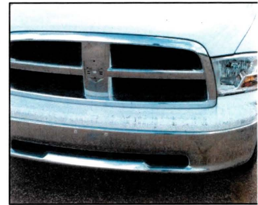
Damage to vehicle after Test Nos. 690900-DTC19-9 through 12.
