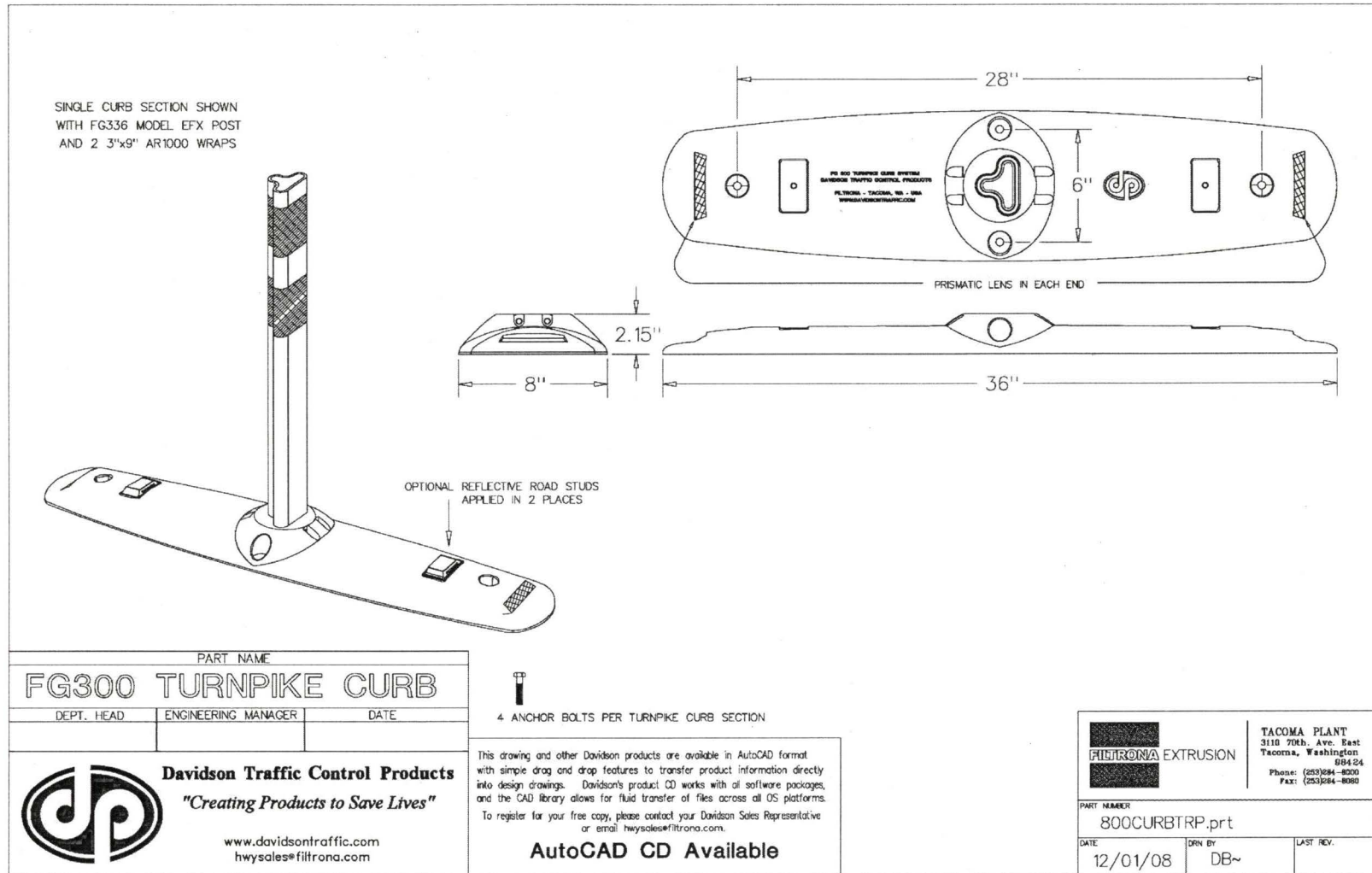
Figure 2.1. Details of the Turnpike Curb System with 36-inch Tall Model EFX.
