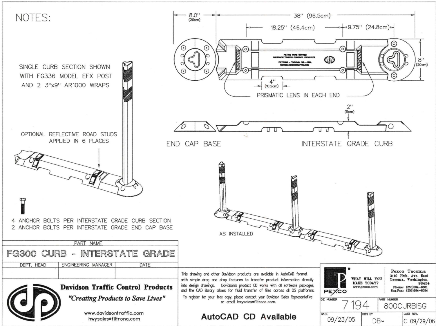
Figure 2.1. Details of the Interstate Grade Curb System with 36-inch Tall Model EFX Post.
