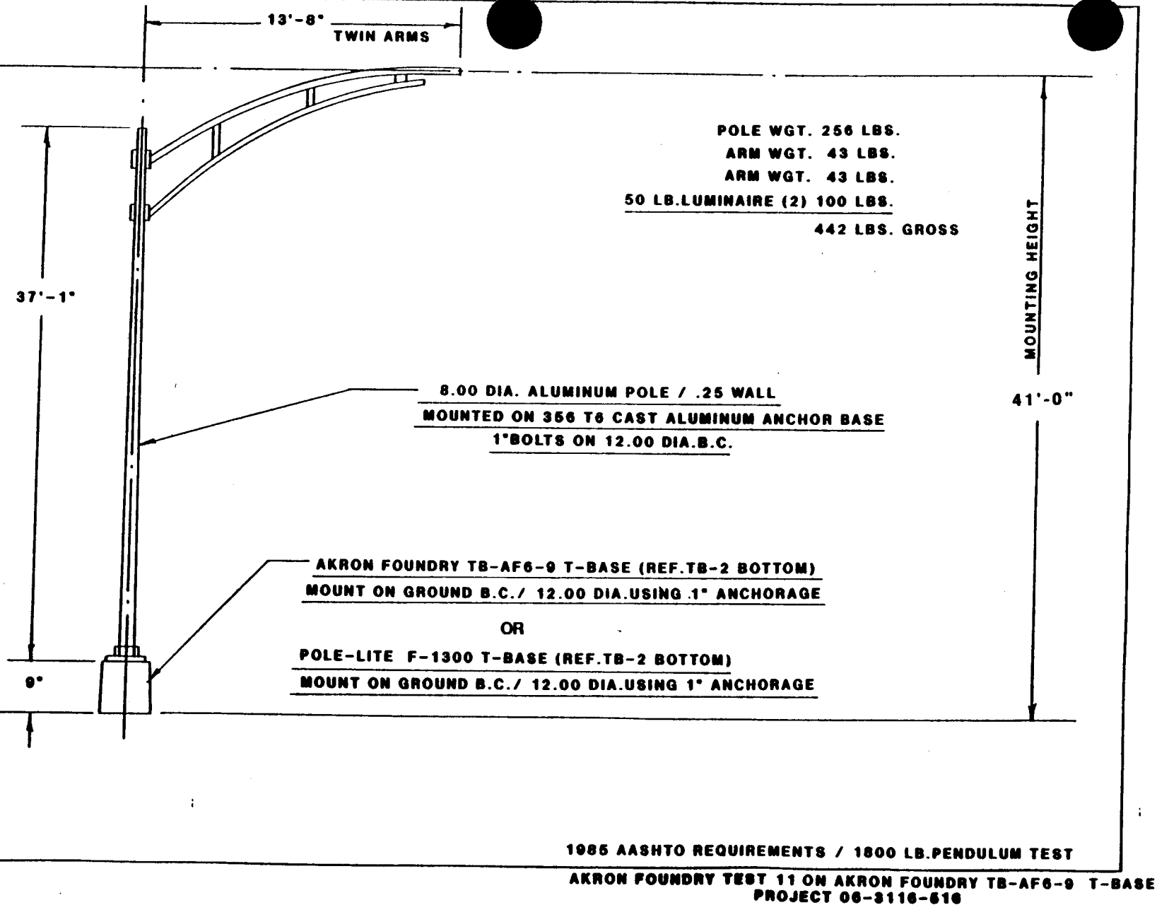
Figure 3. Assembly Drawing, Akron Foundry Test 11
