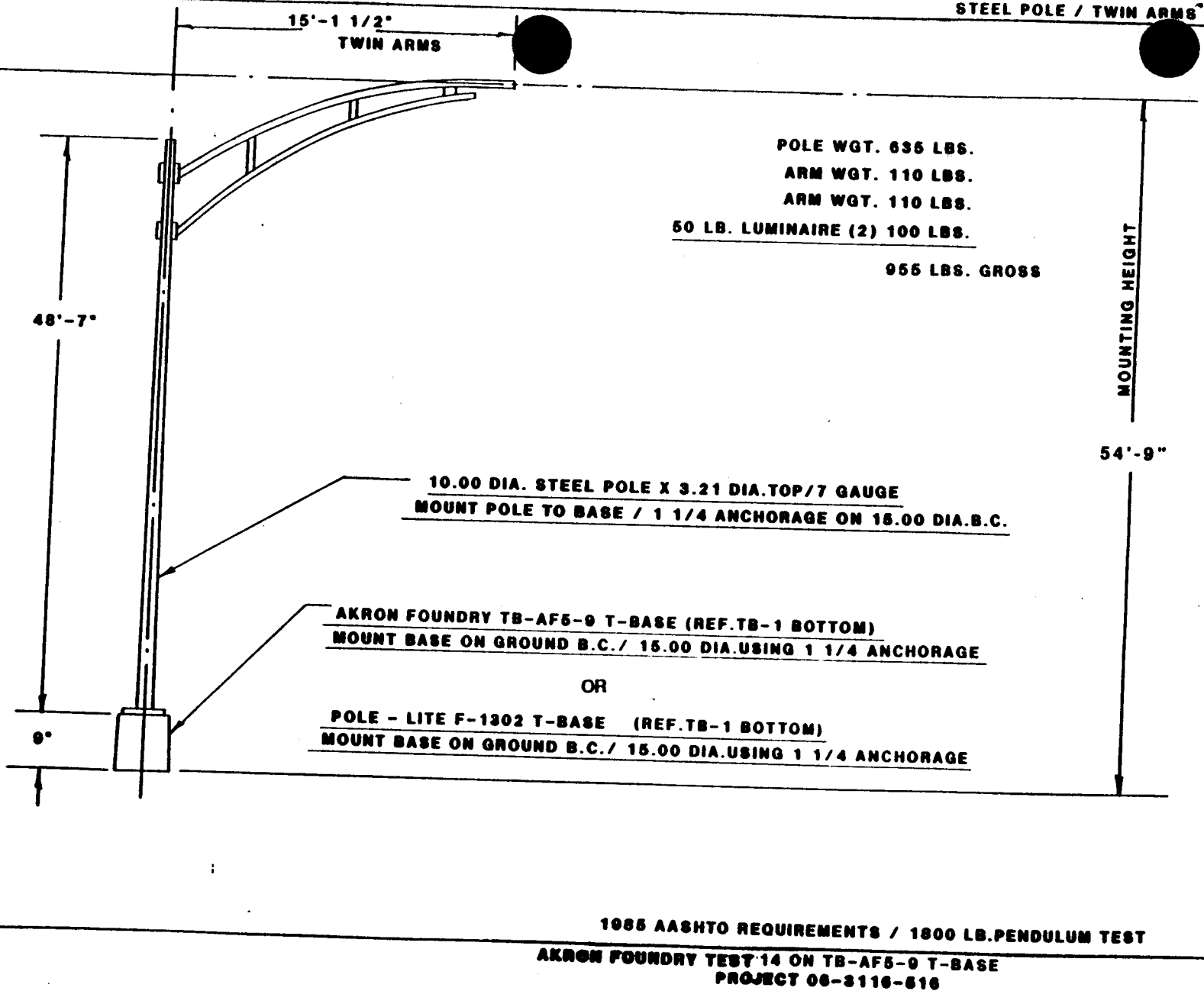
Figure 3. Assembly Drawing, Akron Foundry Test 14
