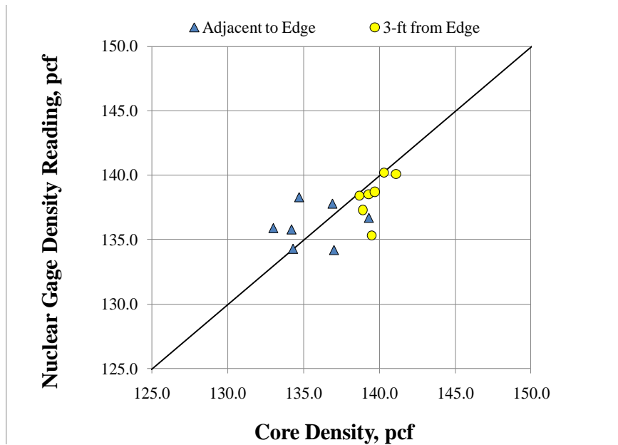
Figure 4. Comparison of the nuclear densities and core densities.
