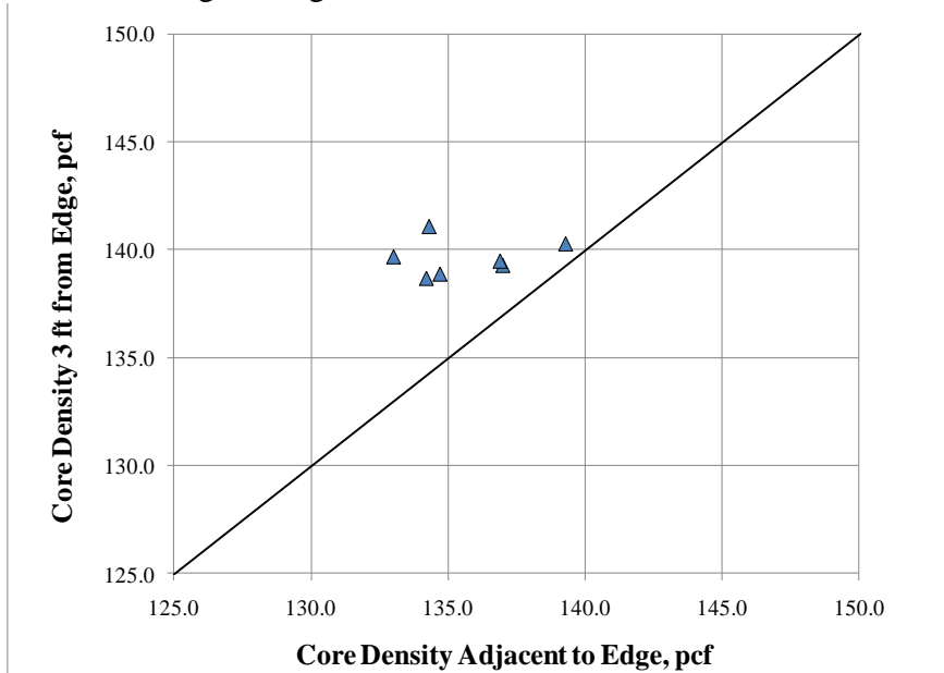
Figure 3. Comparison of core densities adjacent to the edge and 3 feet from the edge.
