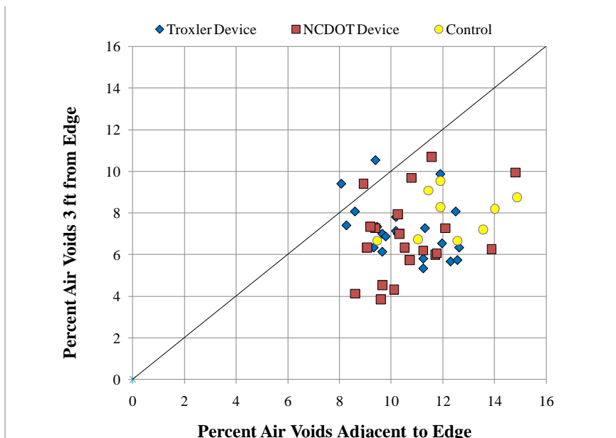
Figure 6. Comparison of the air voids adjacent to the edge and 3 feet from the edge.
