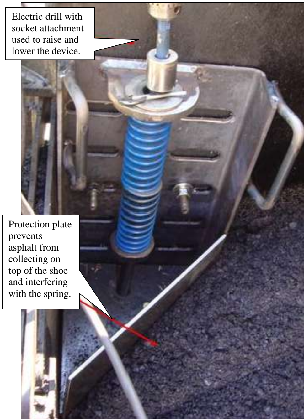
Figure 21. NCDOT second prototype in service showing the protection plate keeping asphalt from collecting on top of the shoe.
