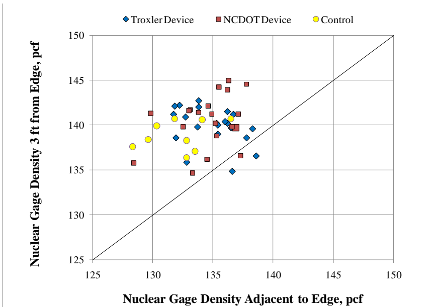
Figure 5. Comparison of the nuclear densities adjacent to the edge and 3 feet from the edge.
