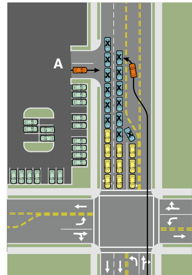
Figure 7: Driveway Location in Relation to Future Traffic Queues on a Major Roadway (Blue Vehicles with X Indicate Future Traffic Queues)
