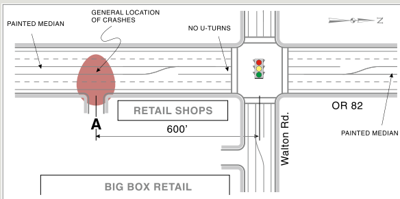
Figure A: Original Driveway and Roadway Configuration
