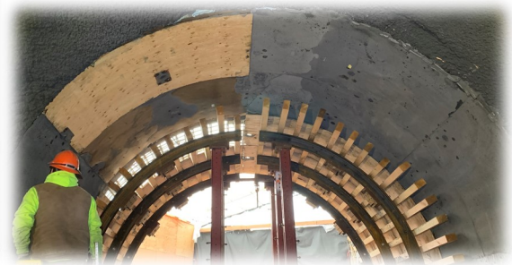
Below: Removing the formwork from the tunnel arch of the East portal
