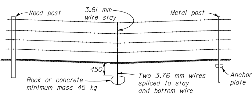
TYPICAL SAG SECTION - TYPE 1 & 2 FENCES
