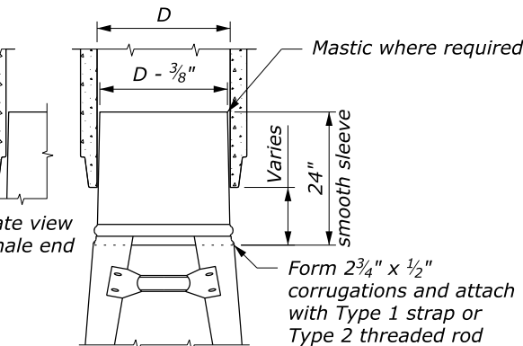
FOR ALL SIZES OF CONCRETE ROUND OR PIPE ARCHES
