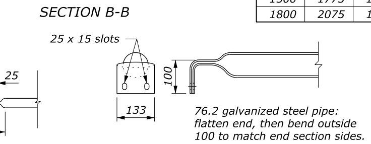
LONGITUDINAL DRAINAGE BAR PARALLEL BARS SAFETY BAR DETAILS NO SCALE
