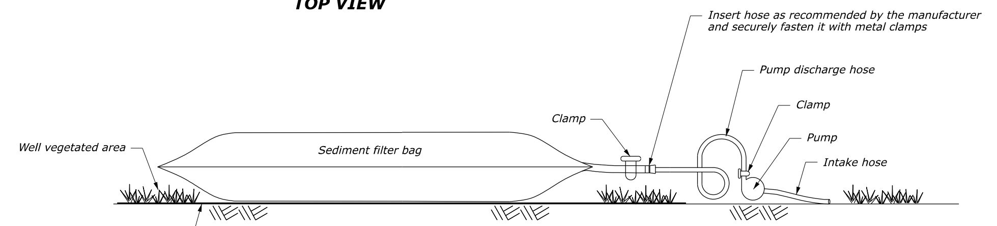
TOP VIEW
