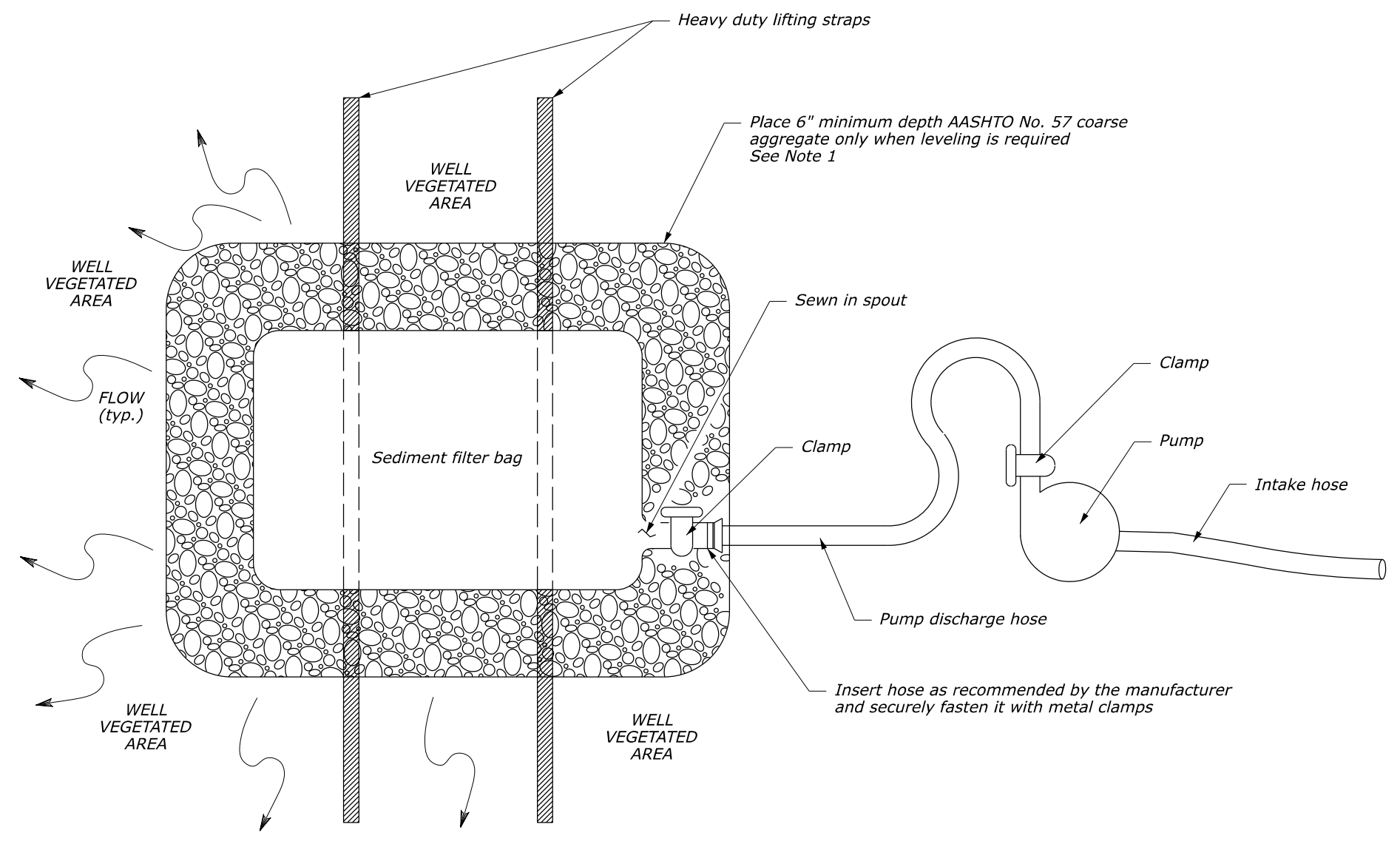
TOP VIEW
