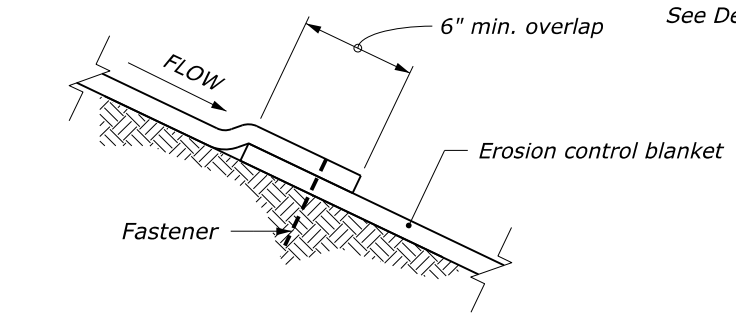
DETAIL C SHINGLE SPLICE
